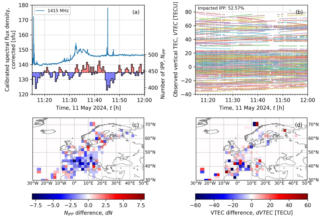
Figure 4. Radio flux and number of ionospheric piercing points n_{\text{IPP}} (a), observed vertical TEC VTEC (b), n_{\text{IPP}} difference map (c) and VTEC difference map (d). The red and blue color coding in panel (a) indicates values greater and smaller than the mean, respectively.
